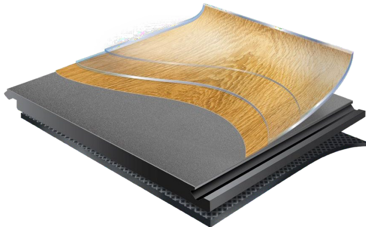
Figure 1: Construction of Kährs LVT SPC Click with PVC Foam Underlayment
