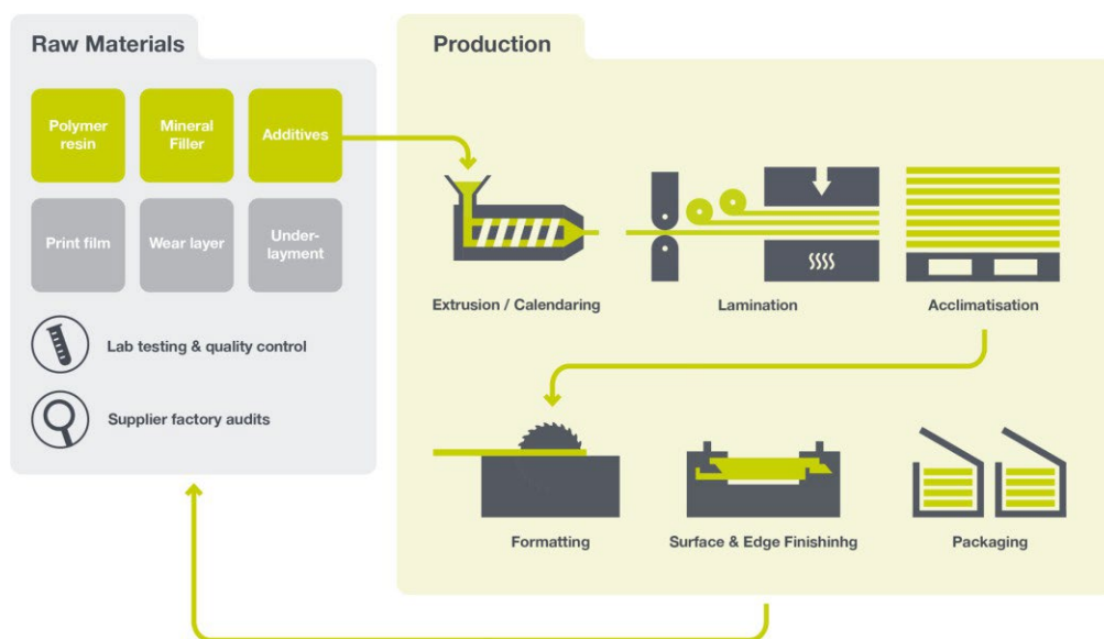
Figure 2: Production Process of Kährs LVT SPC Click with PVC Foam Underlayment
