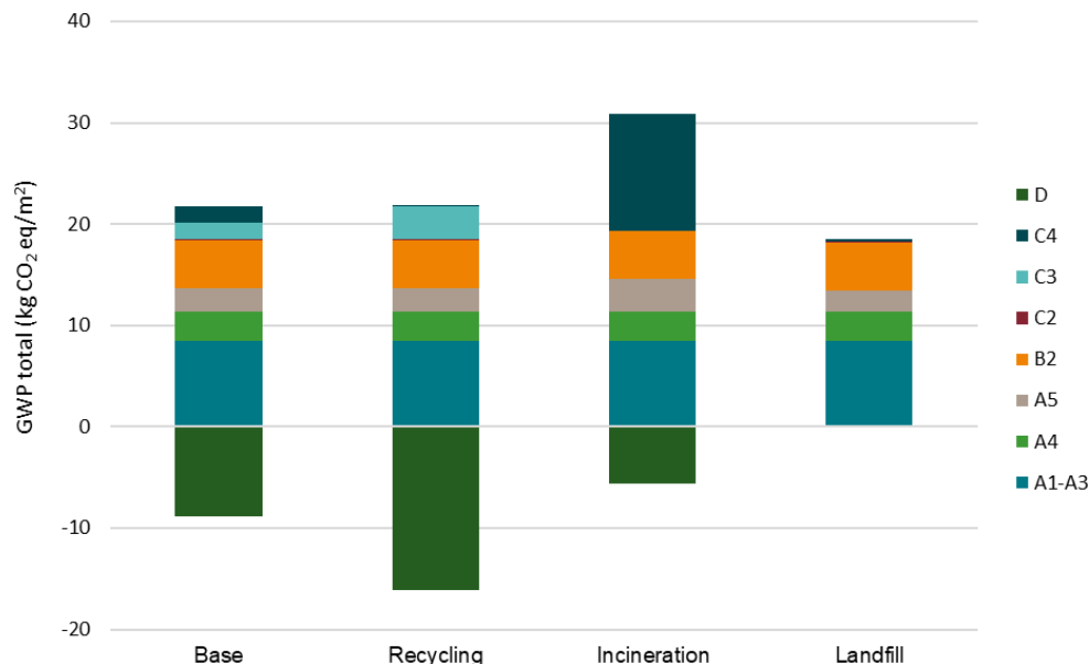
Figure 3: Contributions to GWP for each waste management scenario for SPC Click (excludes B4)
